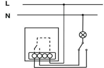
Stairway Switch connection
